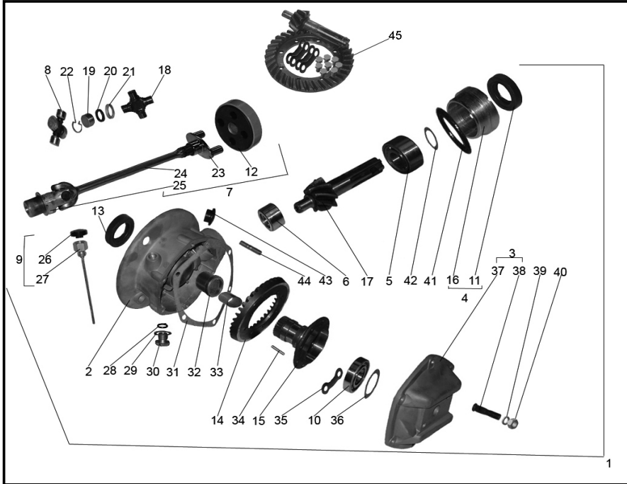
Figure 13. - Final Drive
